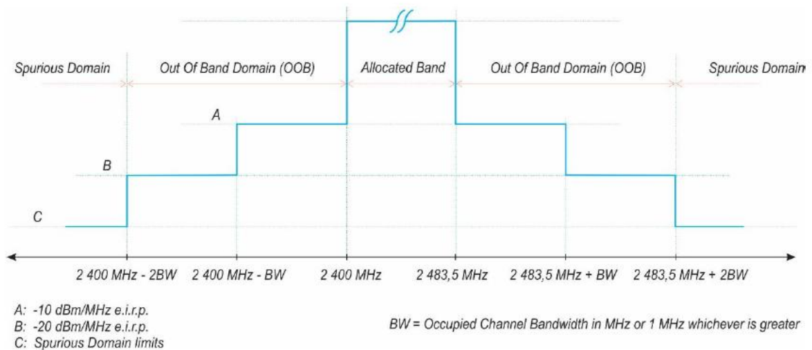
Figure 3: Transmit mask
